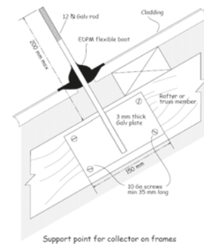
Figure 4: Panel stud fixing
