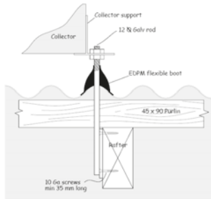
Figure 3: Panel stud fixing
