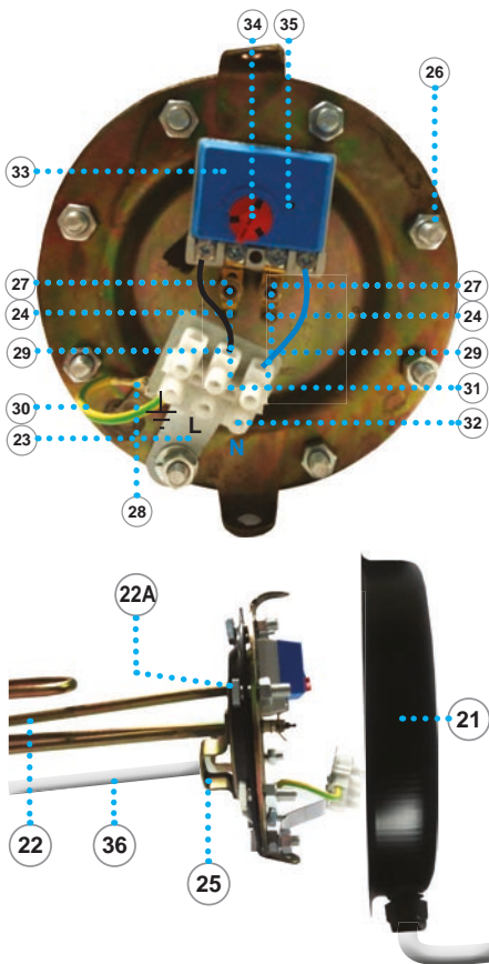
RESISTANCE TYPE "ROUND" DIAGRAM OF ELECTRIC CONNECTION OF THE THERMOSTAT
